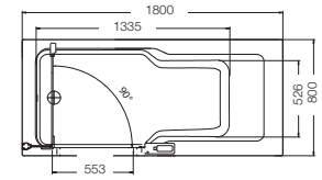
TWINLINE 2 180 x 80 cm Bathtub / Badkuip
