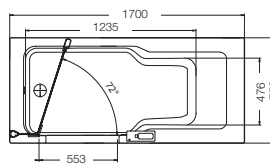
TWINLINE 2 170 x 75 cm Bathtub / Badkuip
