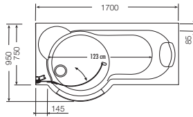
TWINLINE 1 Bathtub / Badkuip 170
